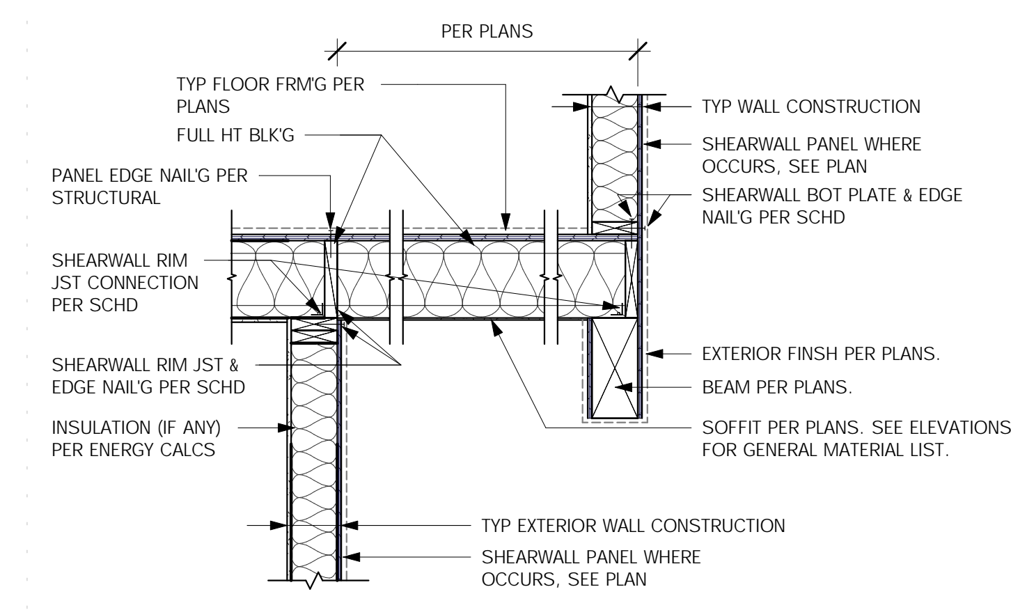
14 CANTILEVER FRM'G AT EXT. WALL SCALE: 3/4" = 1'-0"
