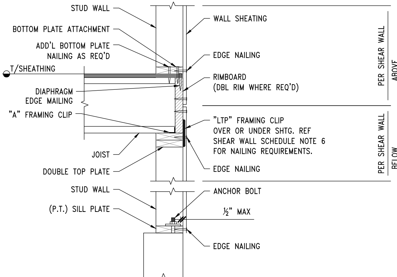
5 DETAIL SCALE: NTS TYPICAL SHEAR WALL SECTION
