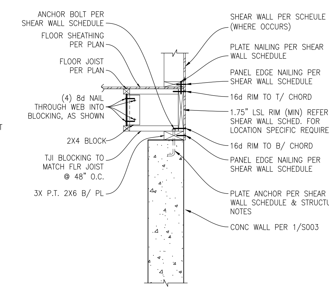
10 DETAIL SCALE: 3/4"=1'-0" TJI PARALLEL TO CONC. WALL
