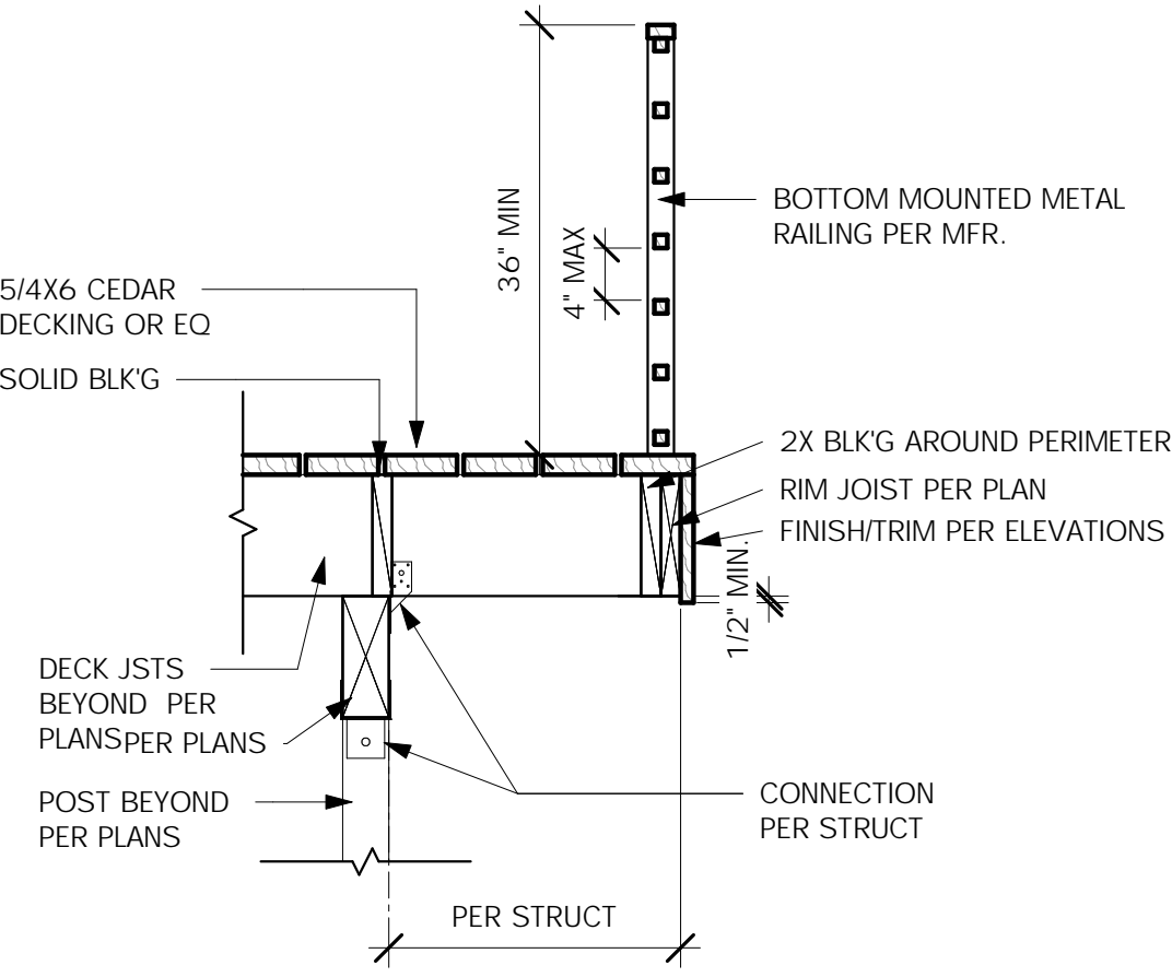
6 FRM'G CONNECTION @ DECK RAILING SCALE: 3/4" = 1'-0"
