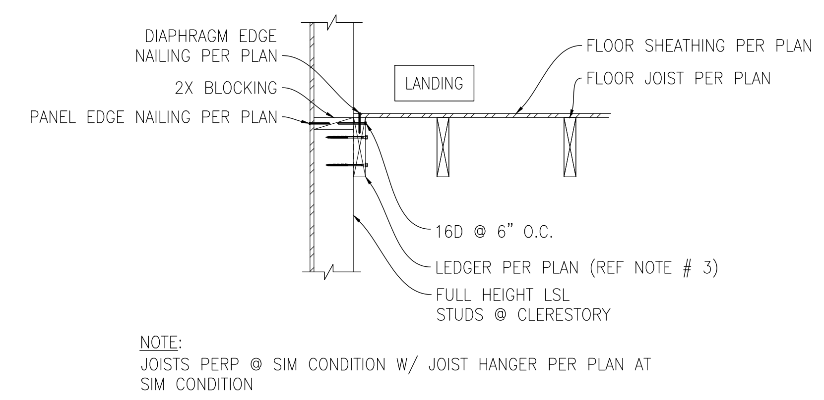
5 DETAIL SCALE: 3/4"=1'-0" TYPICAL LANDING FRAMING
