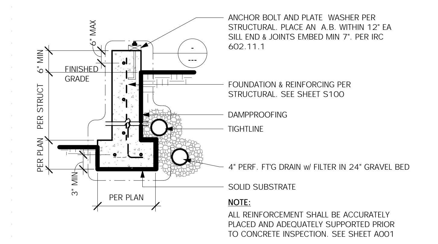
1 FOUNDATION DETAIL SCALE: 3/4" = 1'-0"
