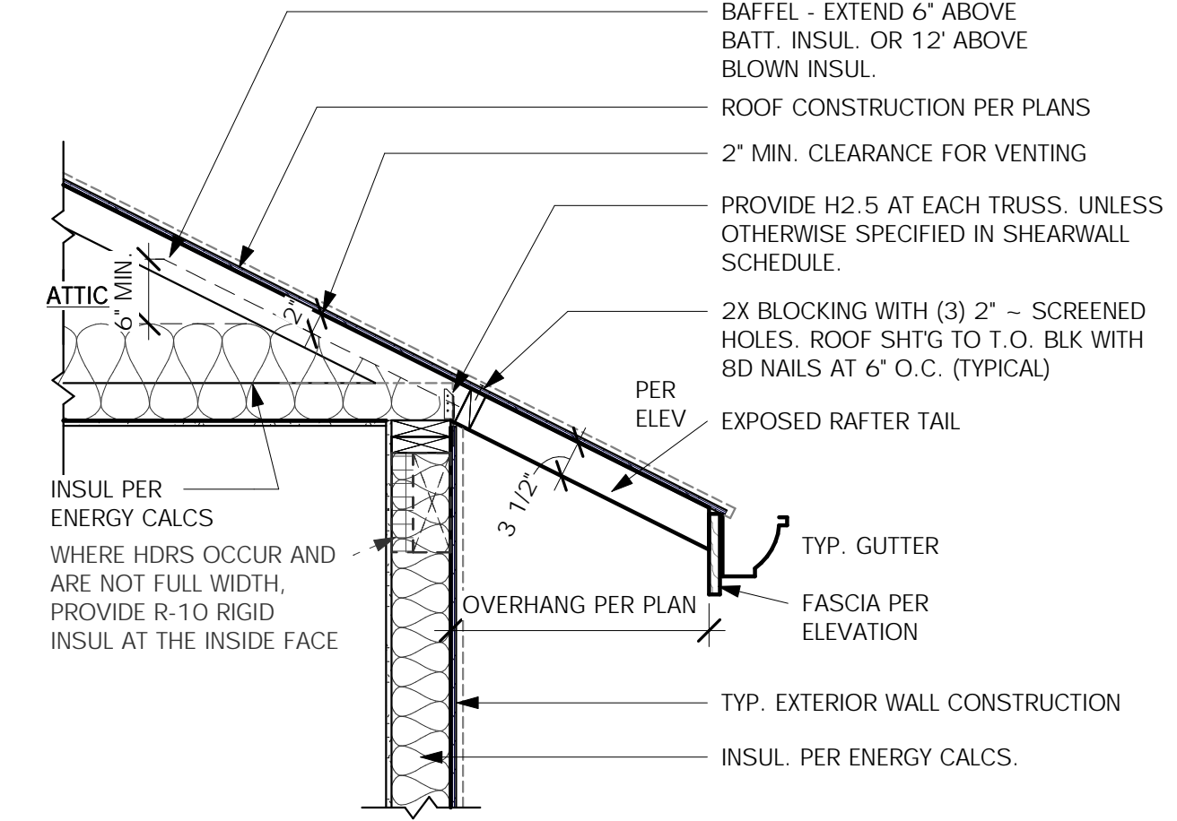
1 EAVE DETAIL - TRUSS SCALE: 3/4" = 1'-0"
