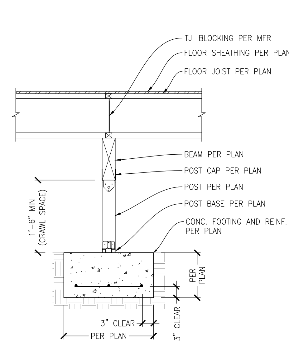
9 DETAIL SCALE: 3/4"=1'-0" ISOLATED POST BASE
