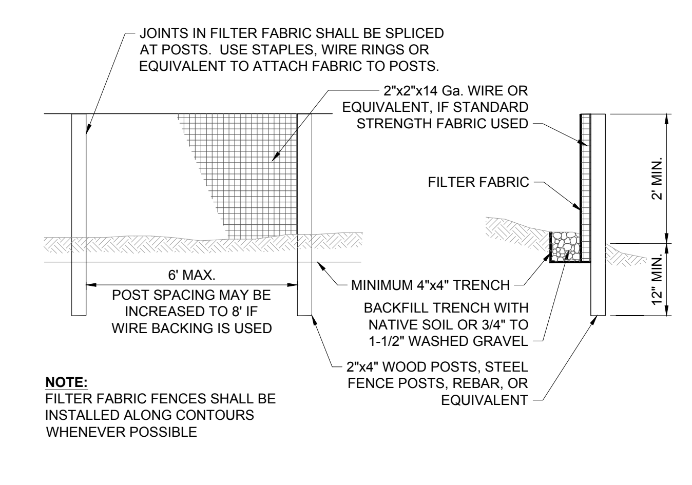
FIGURE D.2.1.3.A SILT FENCE
