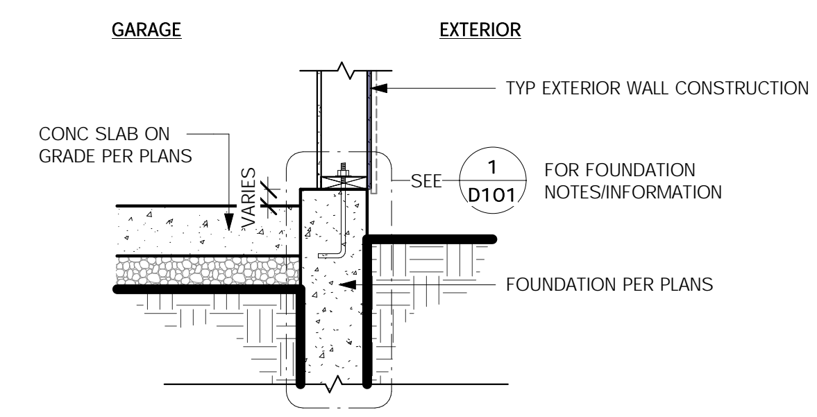
6 SLAB AT STEM WALL SCALE: 3/4" = 1'-0"
