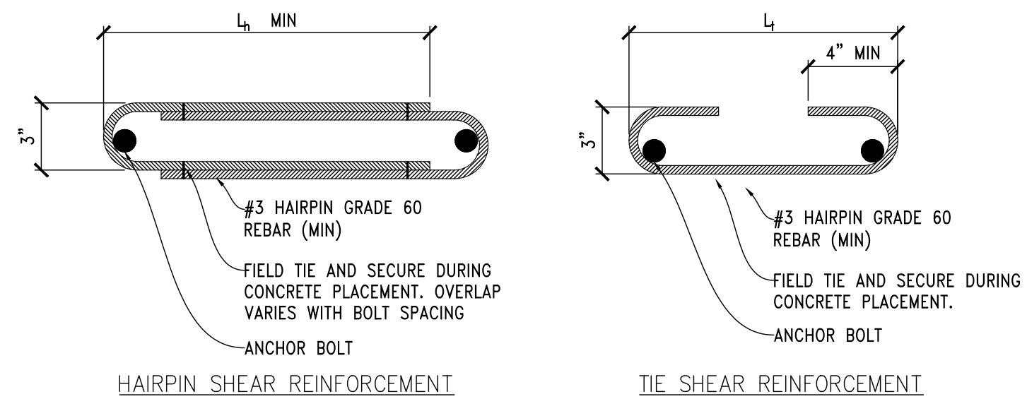
4 DETAIL SCALE: 3/4"=1'-0" TYPICAL STRONGWALL ANCHORAGE - SECTION
