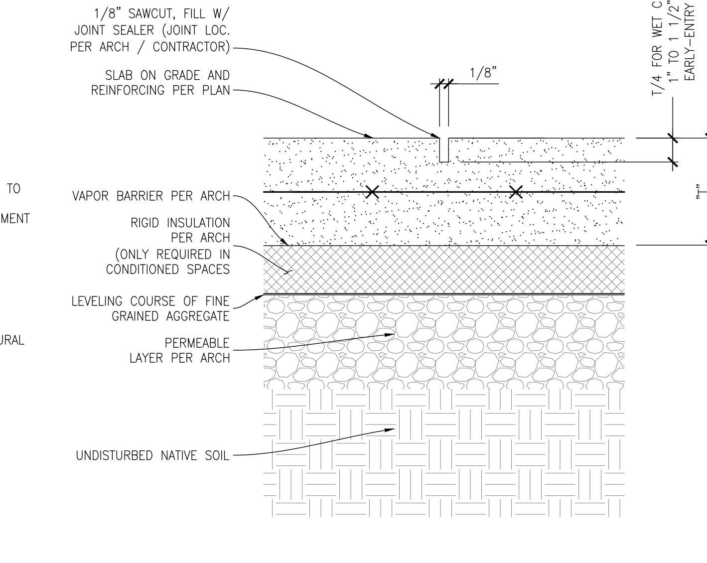
11 DETAIL SCALE: 3/4"=1'-0" TYPICAL SAW CUT JOINT
