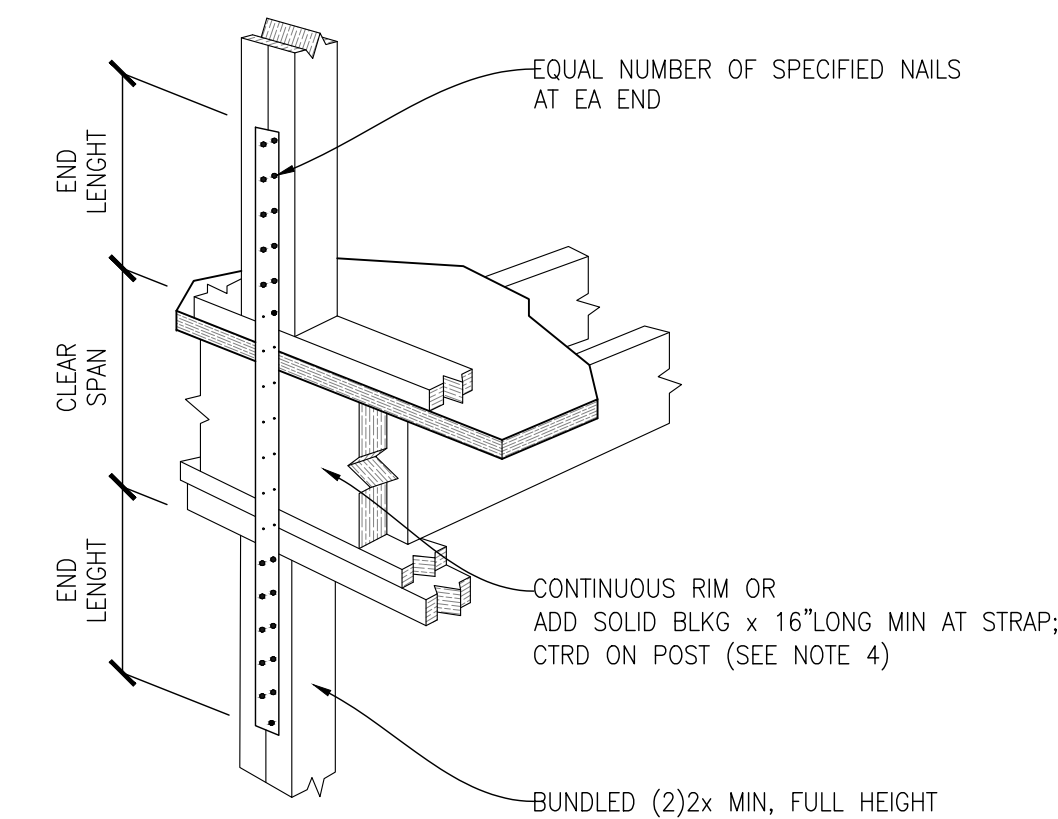
7 DETAIL SCALE: NTS TYPICAL FLOOR TO FLOOR STRAP
