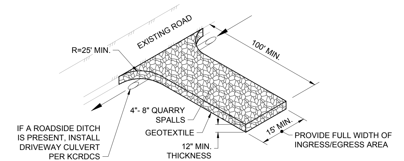
FIGURE D.2.1.4.A STABILIZED CONSTRUCTION ENTRANCE
