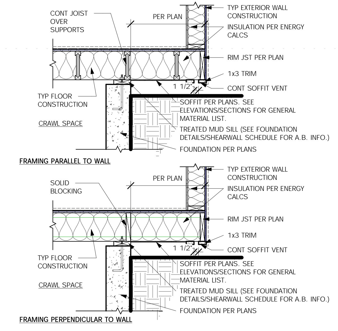
7 CANTILEVER FRM'G AT FNDN. SCALE: 3/4" = 1'-0"
