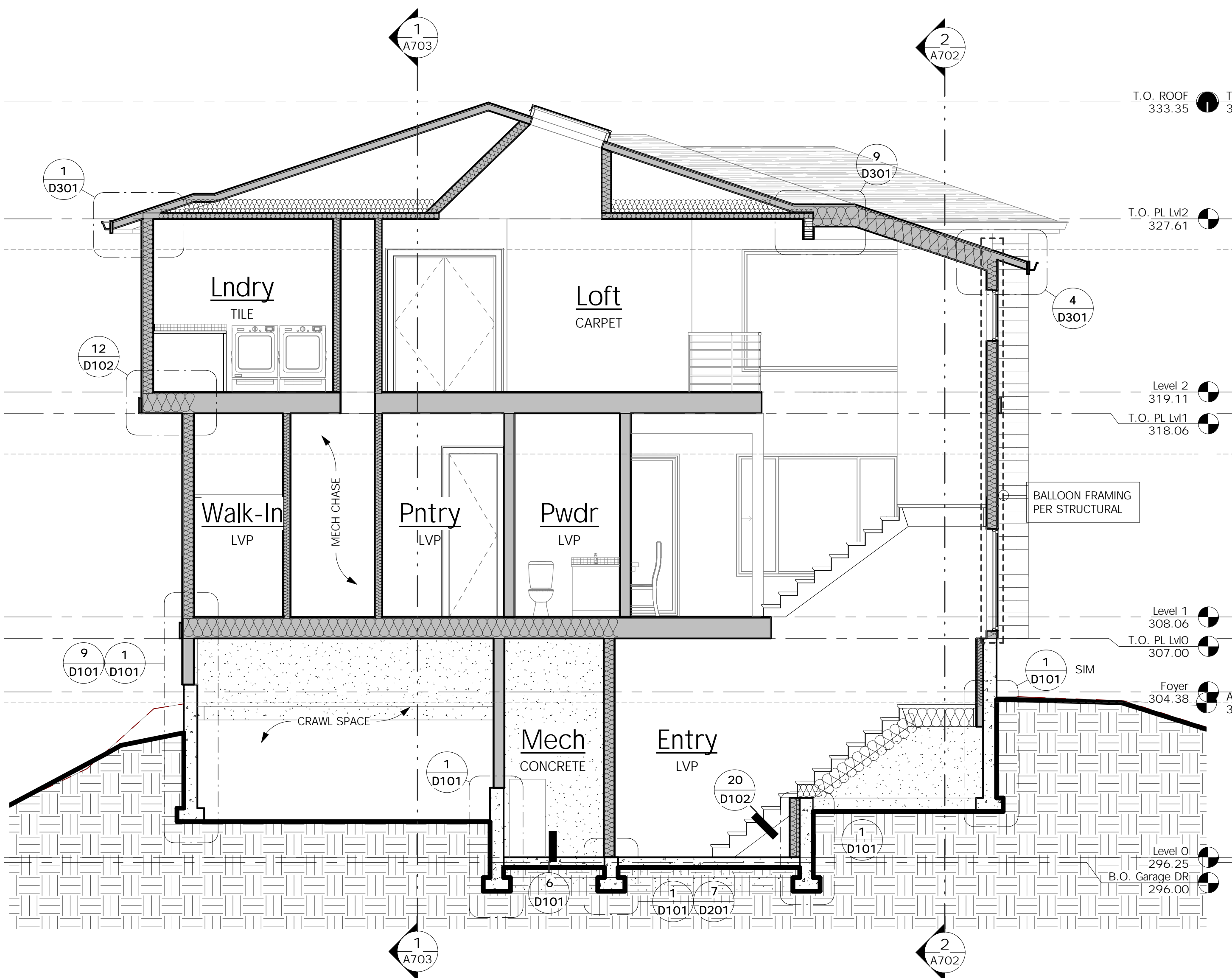
2 Building Section E/W 2 SCALE: 1/4" = 1'-0"
