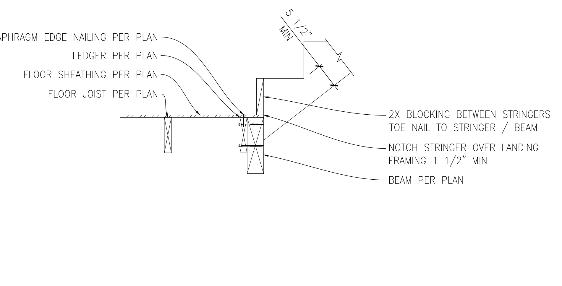
6 DETAIL SCALE: 3/4" = 1'-0" TYPICAL STRINGER FRAMING
