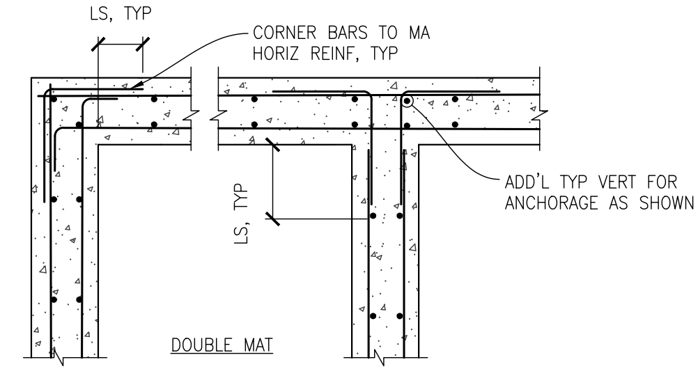
5 DETAIL SCALE: 3/4"=1'-0" TYPICAL CORNER REINFORCING
