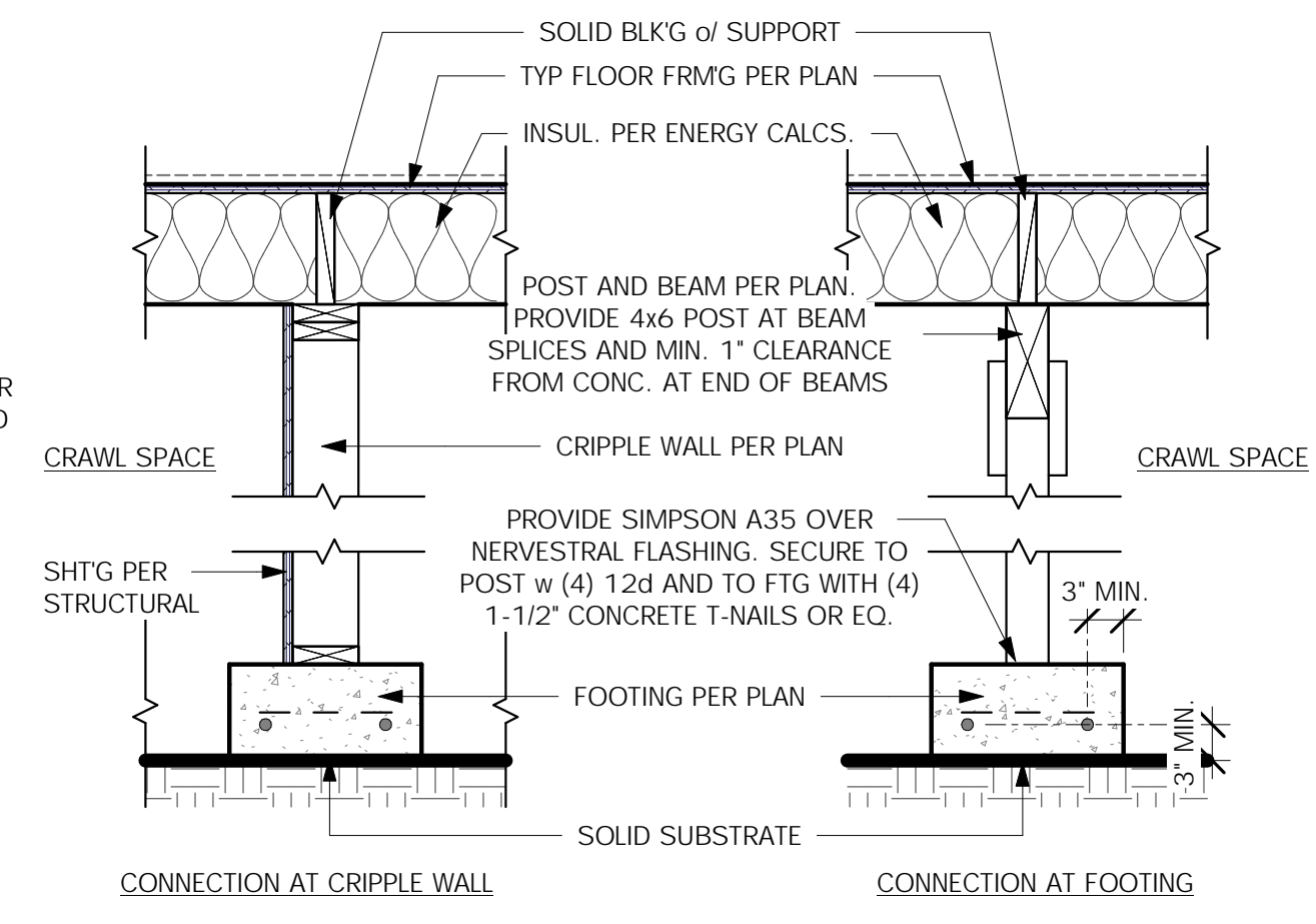
8 POST / FTG CONNECTION SCALE: 3/4" = 1'-0"
