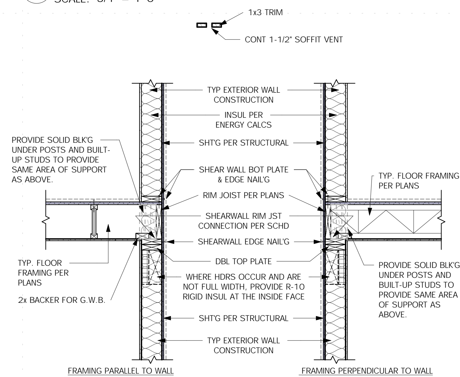
13 EXTERIOR WALL TO FLOOR JOISTS SCALE: 3/4" = 1'-0"
