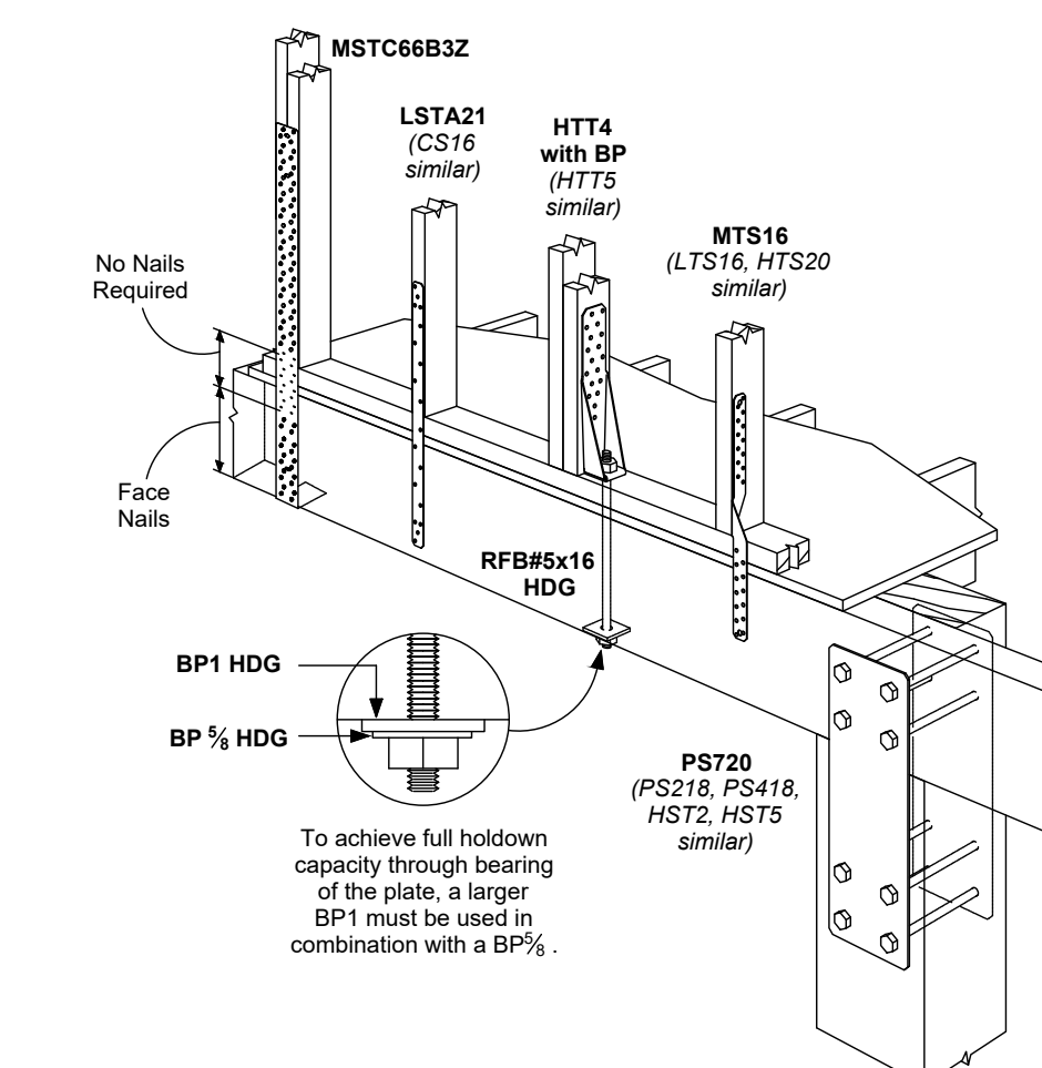
8 DETAIL SCALE: NTS FLOOR TO BEAM / RIM HOLDDOWNS
