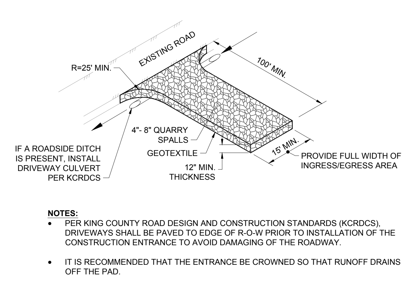
FIGURE D.2.1.4.A STABILIZED CONSTRUCTION ENTRANCE
