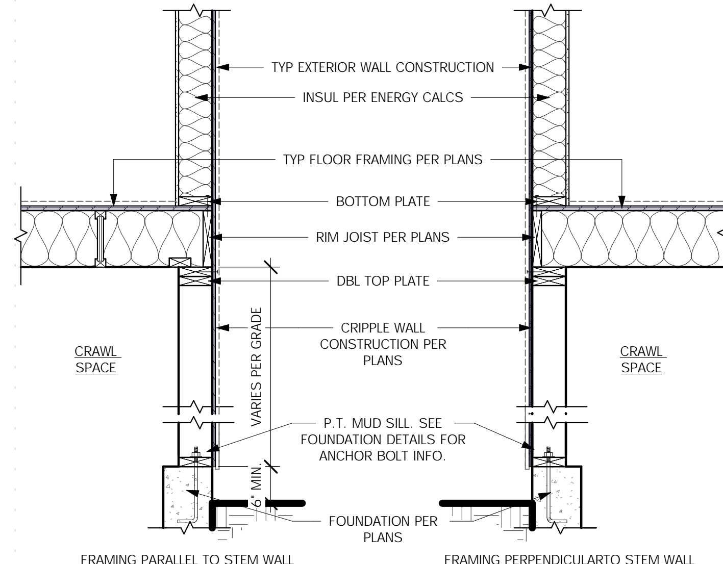
9 CRIPPLE WALL AT FOUNDATION SCALE: 3/4" = 1'-0"
