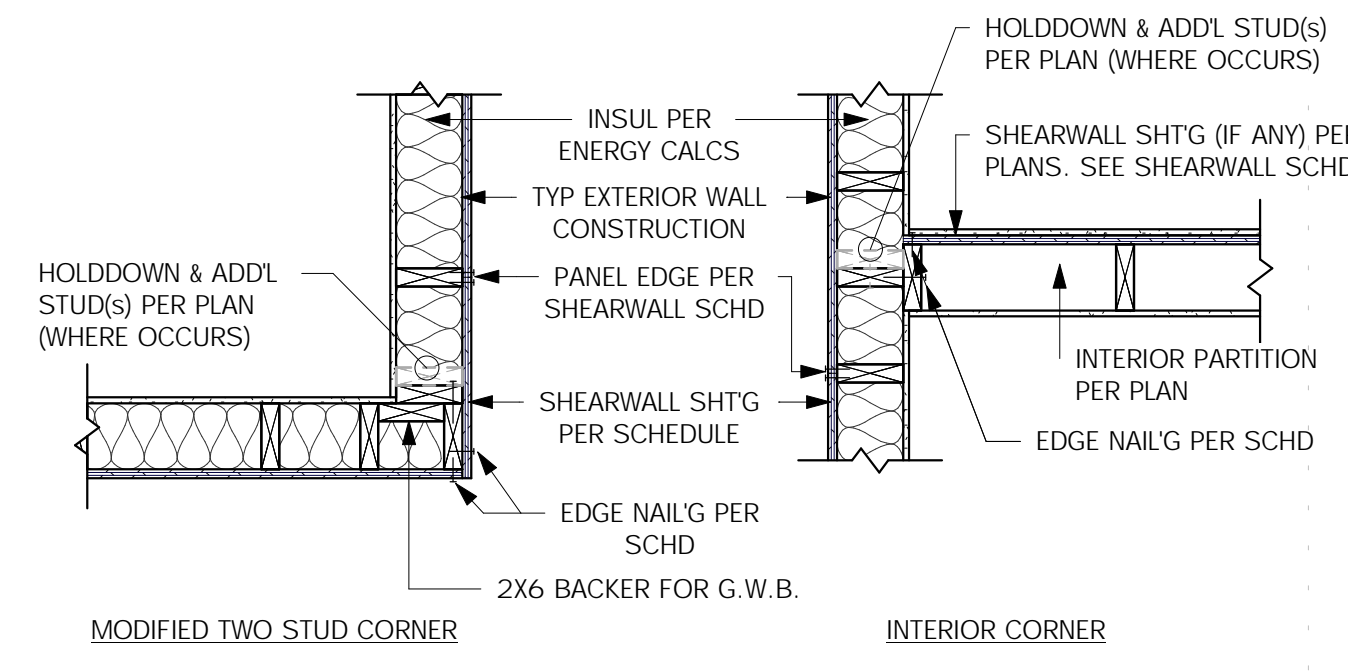
11 INT/EXT WALL FRAMING DETAIL SCALE: 3/4" = 1'-0"
