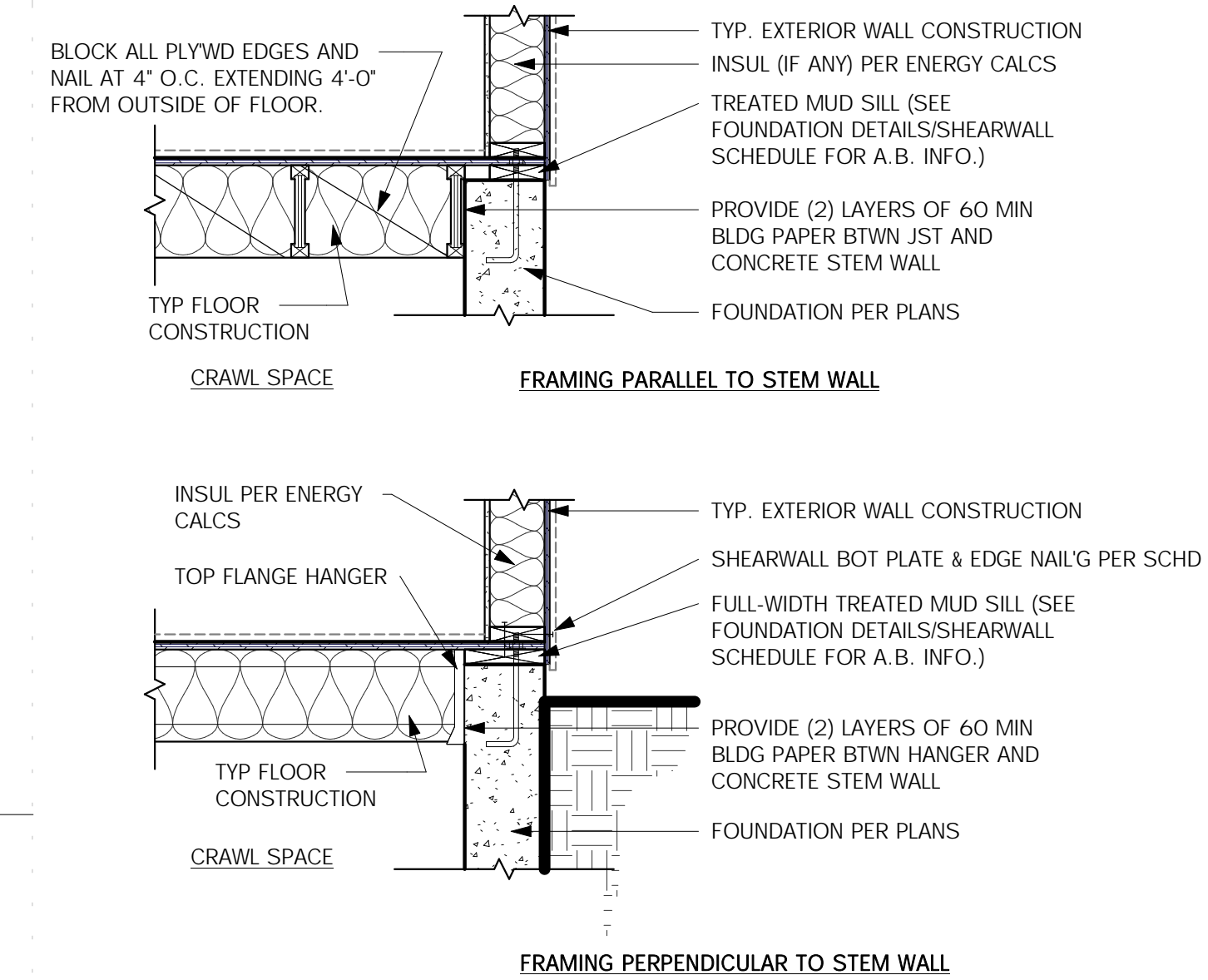
3 FRAMING / FNDN. CONNECTION SCALE: 3/4" = 1'-0"
