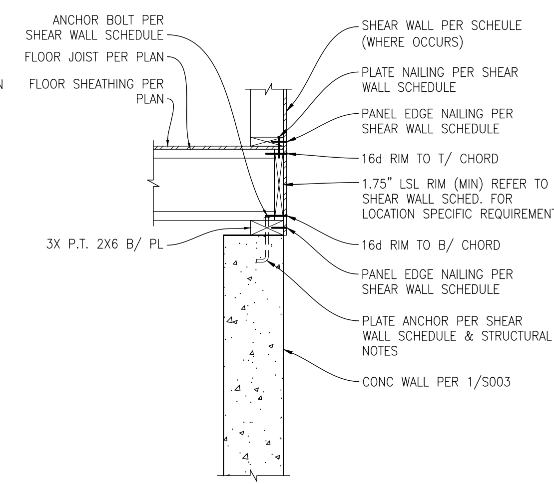
10 DETAIL SCALE: 3/4"=1'-0" TJI PERP. TO CONC. WALL
